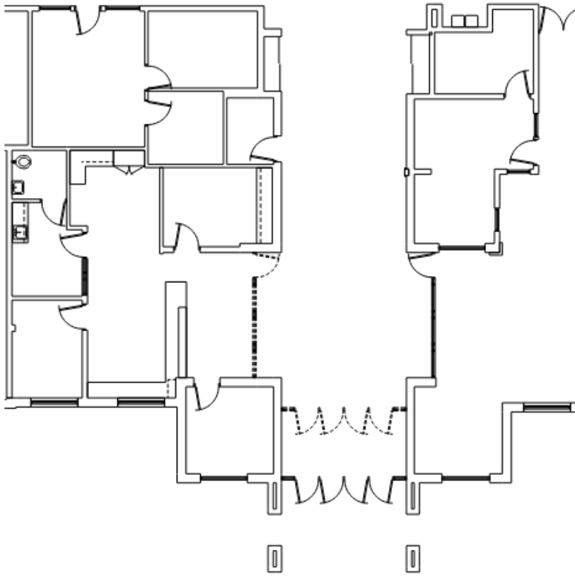
DEMOLITION - PARTIAL FIRST FLOOR PLAN
